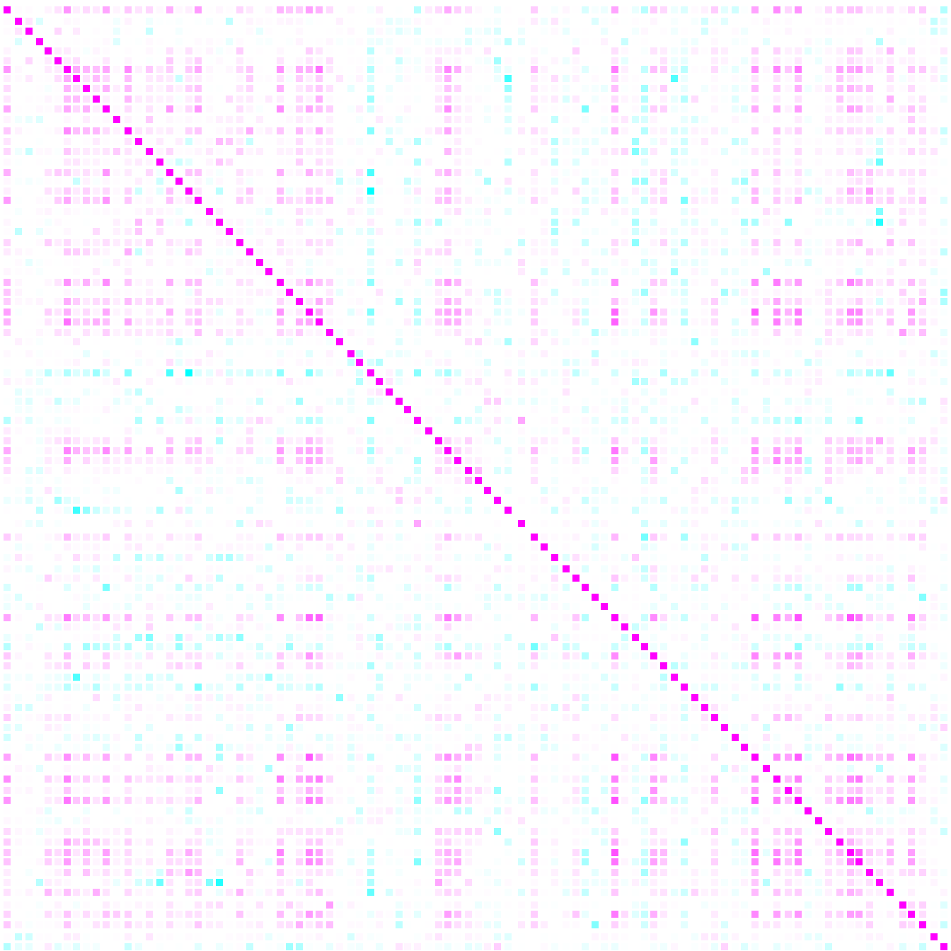
Correlation matrix
