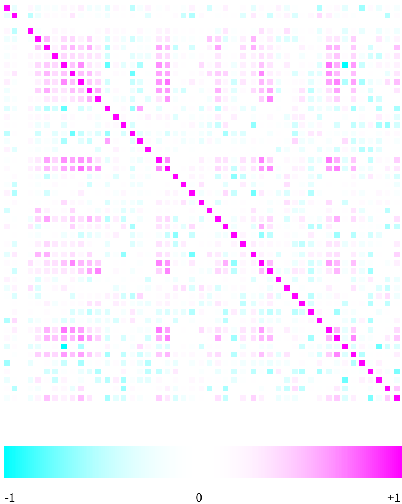
Correlation matrix
