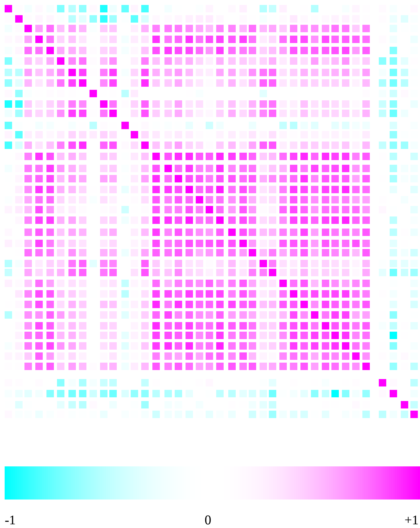
Correlation matrix
