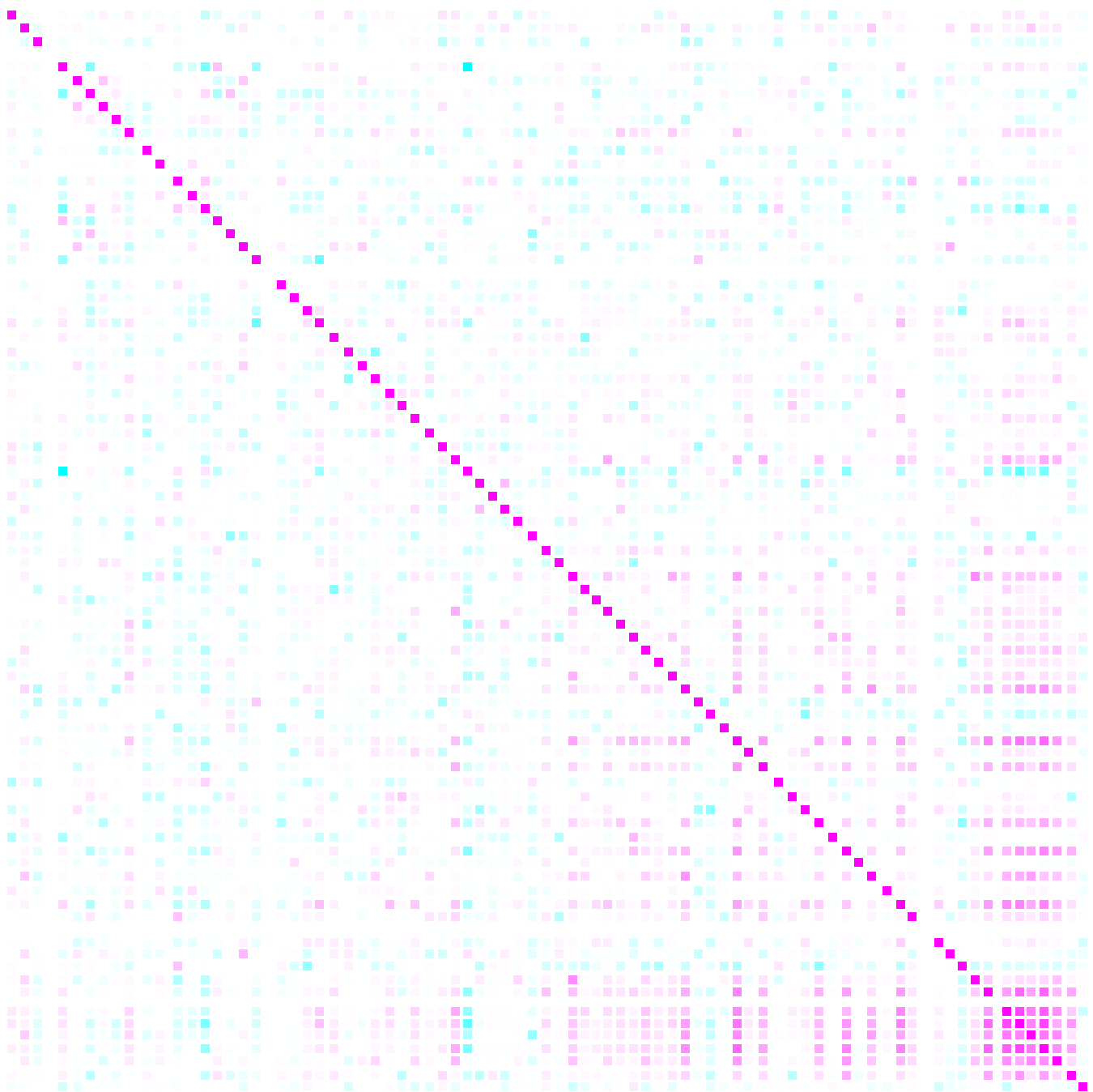
Correlation matrix
