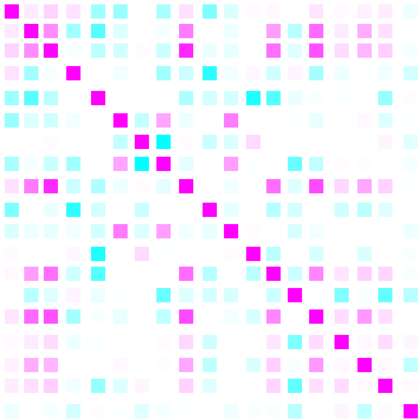
Correlation matrix
